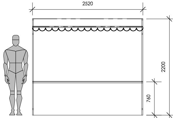
FRONT EXTERNAL VIEW B - B
